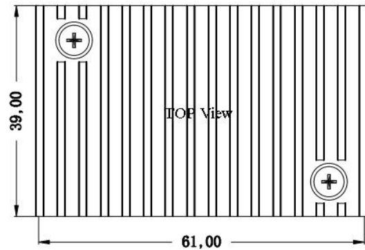
Standard+Heatsink 61.0*39.0*27.7mm
