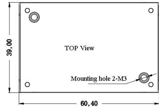
Standard 60.4*39.0*12.7mm
